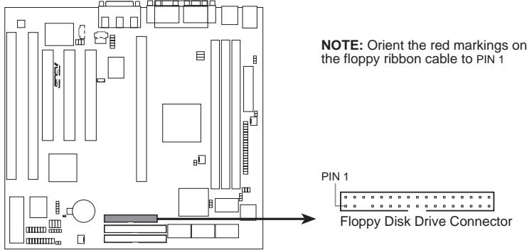
P2L-VM/P2E-VM Floppy Disk Drive Connector
